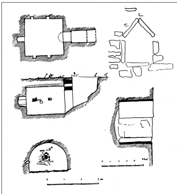
Сл. 5. Сврљиџ, гробница у цркви Св. Стефана (према Ђ. Бошковић) Fig. 5. Svrljig, the crypt in the former church of St Stephan (according to Dj. Bošković)
