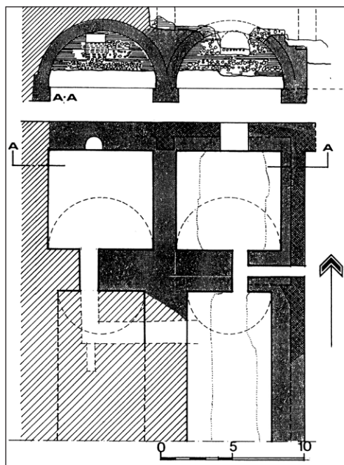
Fig. 3 Niš, central area of the Turkish fortress, the ground plan and cross-section view of the building under vaults (documentation of the Archaeological Institute in Belgrade)
